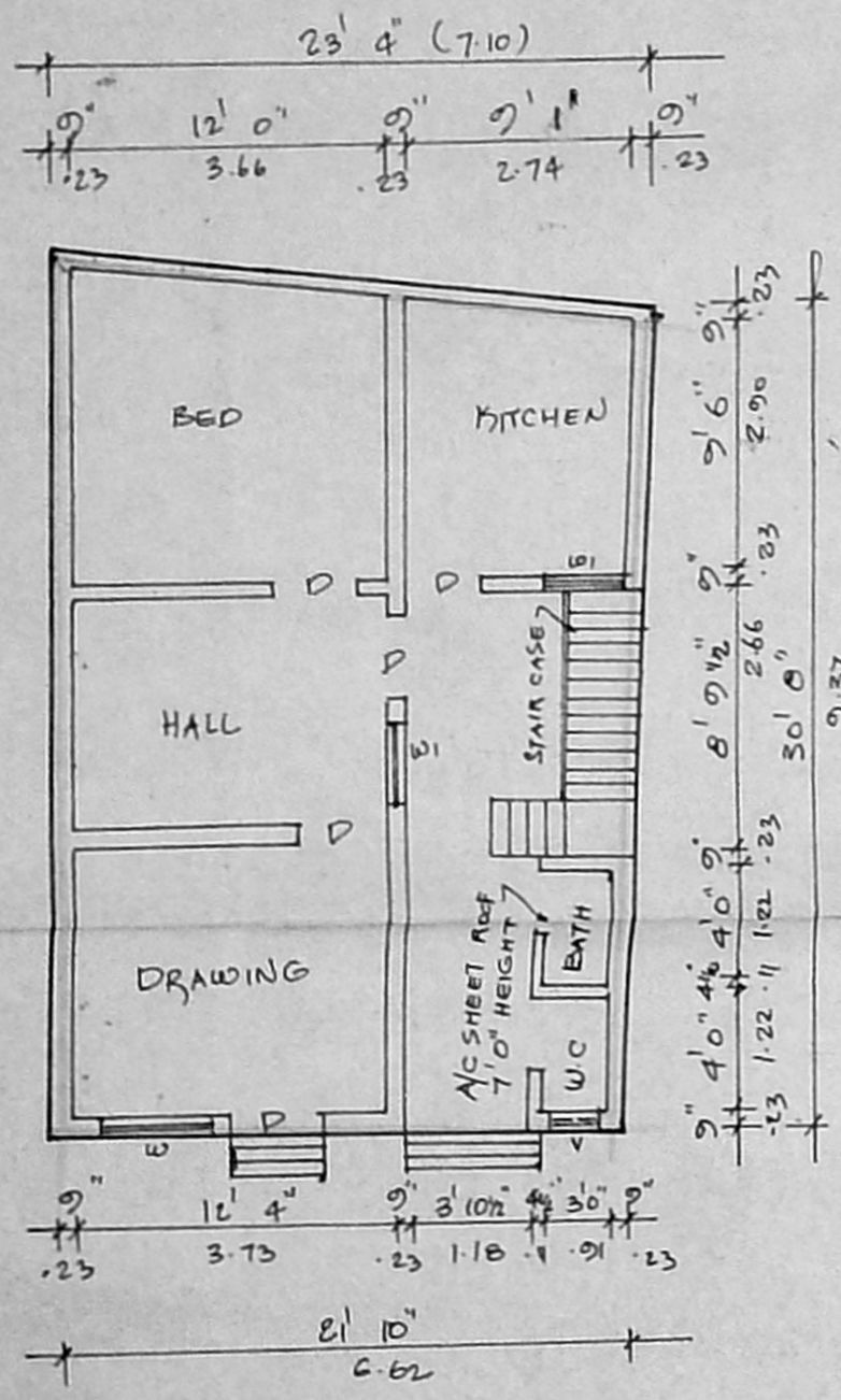
SITE CUM GROUND FLOOR PLAN
