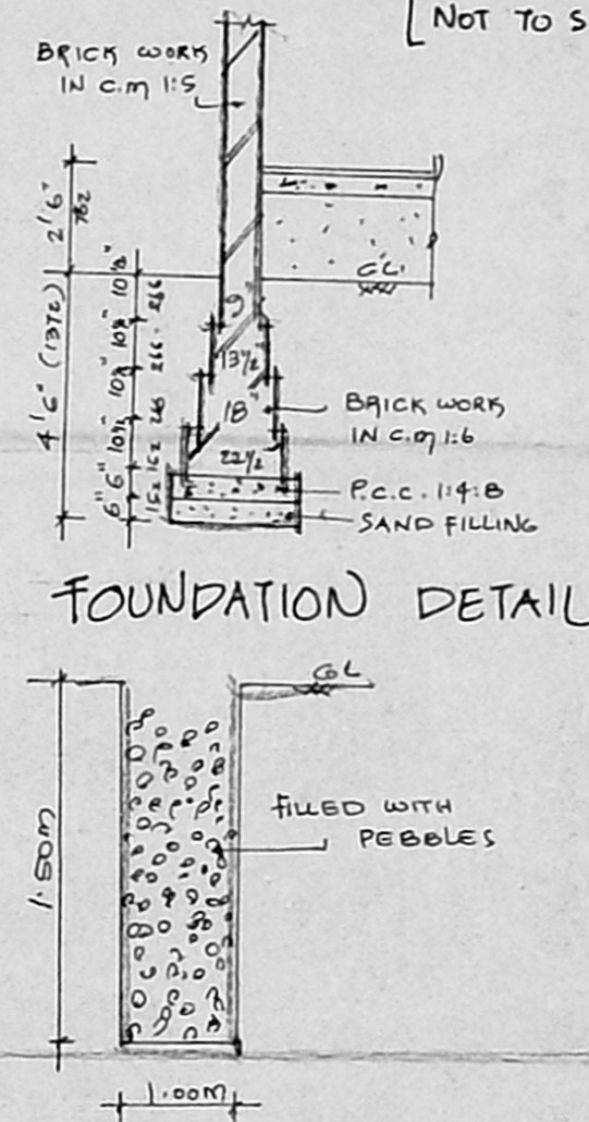
SECTION OF RAIN WATER PERCOLATION PIT
